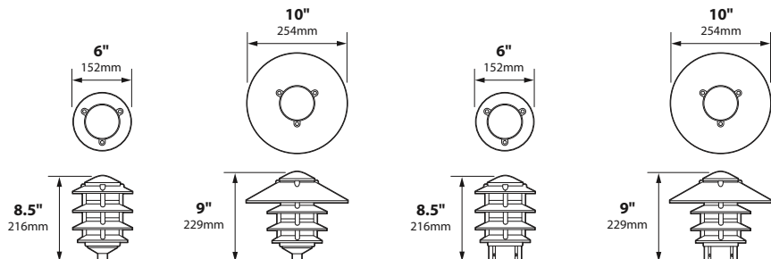
FAL-04-5-120V FAL-04-7-120V FAL-04-9-120V
