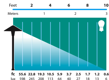
AL-16 Half Spread Photometrics 20 ft. (6.1m) diameter
