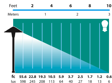
AL-15 Half Spread Photometrics 20 ft. (6.1m) diameter
