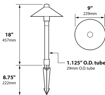
AL-13-DM-CAV 18w Lamp (25w max.) Solid Copper
