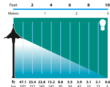
AL-14 Half Spread Photometrics 20 ft. (6.1m) diameter
